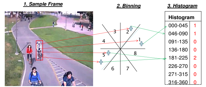
Figure 2: Construction of an Oriented Optical Flow Histogram.
