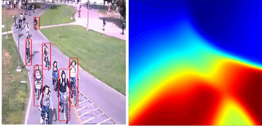
Figure 4: [Best Viewed in Color] Depth/Velocity Normalization, (left) a frame from the video having severe depth disparity. (right) normalized velocity map using kernel regression
