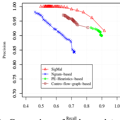
Figure 11: Comparison of malware detection methods with a live malware feed (2012-12-01).
